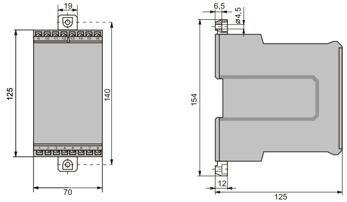
Fig. 4. RISH Ducer P11 in housing E16 with the screw hole brackets pulled out for wall mounting.
