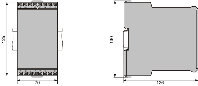
Fig. 3. RISH Ducer P11 in housing E16 clipped onto a top hat rail (35 x 15 mm or 35 x 7.5 mm, acc. to EN 50 022).
