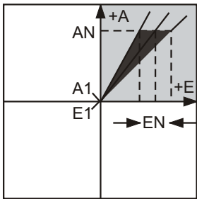
Characteristic 'D' Input E1...EN \pm 10\% Output A1...AN
