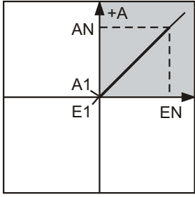
Characteristic 'A' Input E1...EN Output A1...AN
