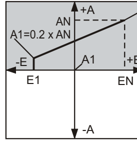
Characteristic 'G' Input E1...EN Output A1...AN
