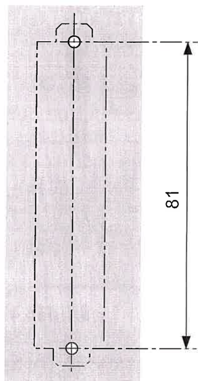
Fig. 5. Drilling plan
