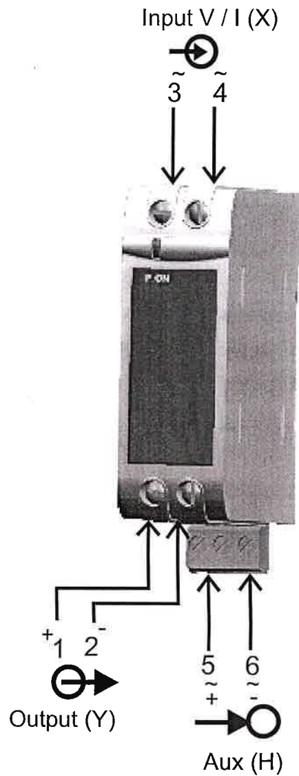
Fig. 6. Front View of Device for electrical Connections
