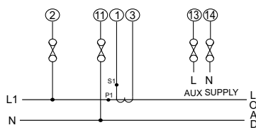
1 Phase 2 Wire
