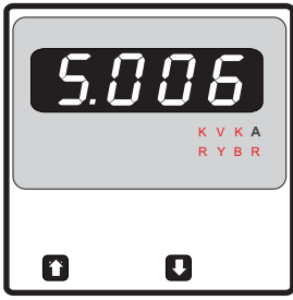
Screen 5 : System Current Max. Value Value displayed after "Hi" flashing on Display
