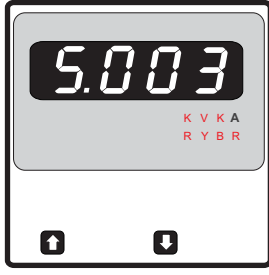
Screen 6 : System Current min. Value Value displayed after "Lo" flashing on Display
