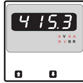
Screen 8 : System Voltage max Value Value displayed after "Hi" flashing on Display
