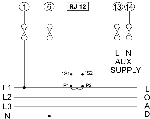
c) Single Phase Load
