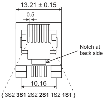
Meter Side RJ 12 Connection
