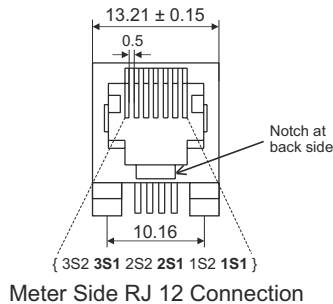
Meter Side RJ 12 Connection
