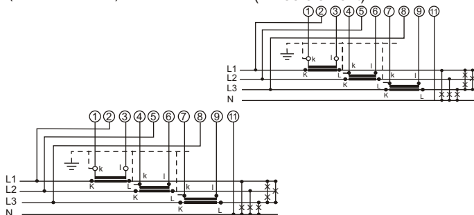
V3W -Three phase, four-wire AC Supply with unbalanced load (Three element)
