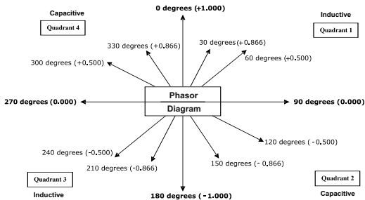
PHASOR DIAGRAM
