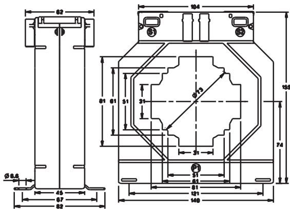
RISH XMER PROTECTION CLASS 140/80 (45)
