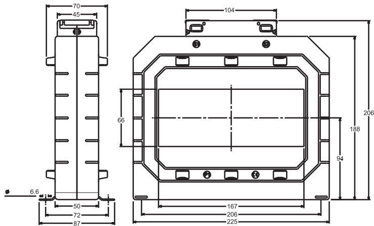
RISH XMER PROTECTION CLASS 225/167 (50)
