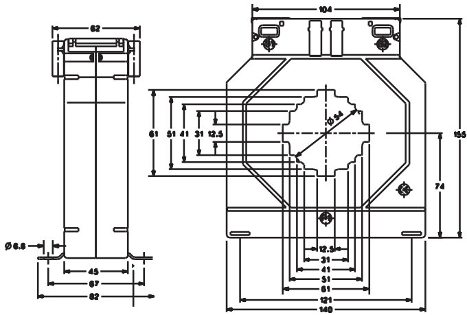
RISH XMER PROTECTION CLASS 140/60 (45)
