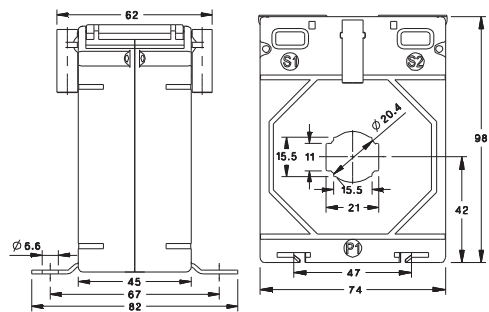
RISH XMER PROTECTION CLASS 74/40 (45)
