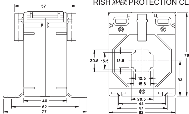
RISH XMER PROTECTION CLASS 62/20 (40)
