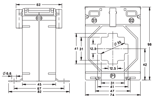
RISH XMER PROTECTION CLASS 74/40 (45)
