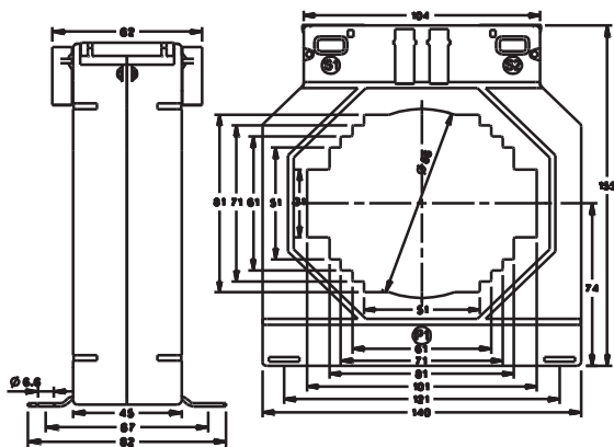
RISH XMER PROTECTION CLASS 140/100 (45)
