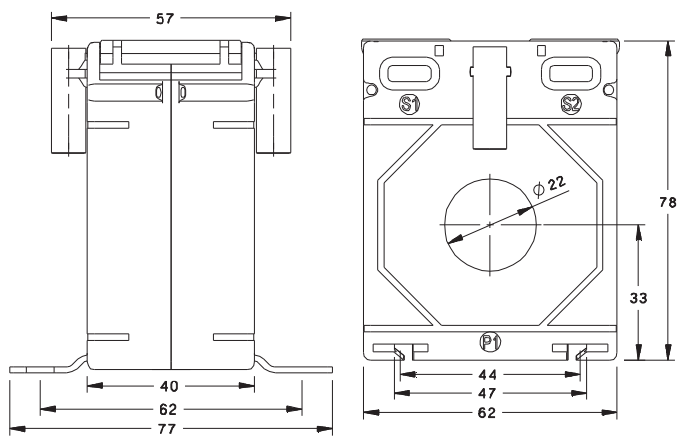
RISH XMER PROTECTION CLASS 62/R
